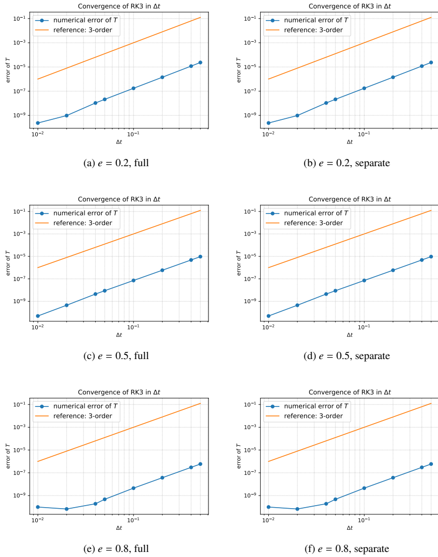
Figure 1: Convergence test in time of the 2D Maxwell molecule (isotropic solution) for e = 0.2, 0.5 and 0.8 , and for both the “full” and “separate” methods. Errors shown here are |T_{\text{num}} - T_{\text{ref}}| at t_{\text{final}} = 2 . N = 64 , N_p = 30 , M_{\text{cir}} = 30 , R = 7.8 , L = 8.61 .
